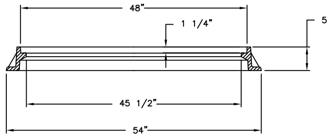
FRAME SECTION
