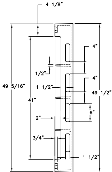
BACK ELEVATION
