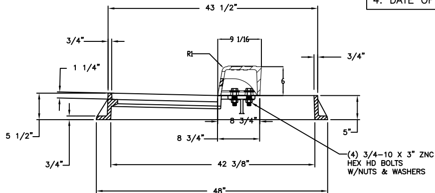
FRAME & BACK SECTION
