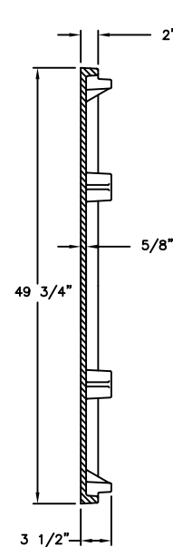
PLATE SECTION
