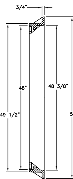
FRAME SECTION
