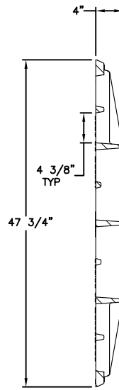
GRATE SECTION
