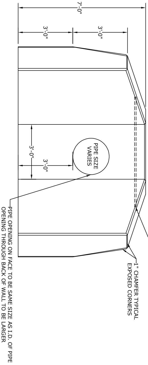
FRONT ELEVATION
