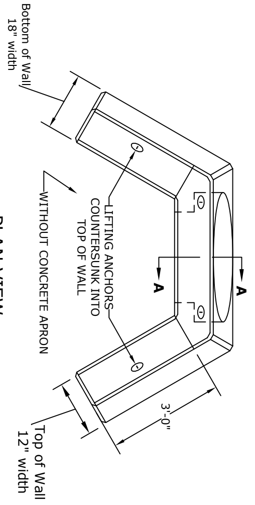
PLAN VIEW
