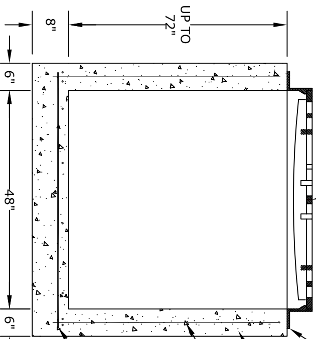
SECTION A
