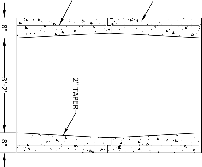
SECTION B
