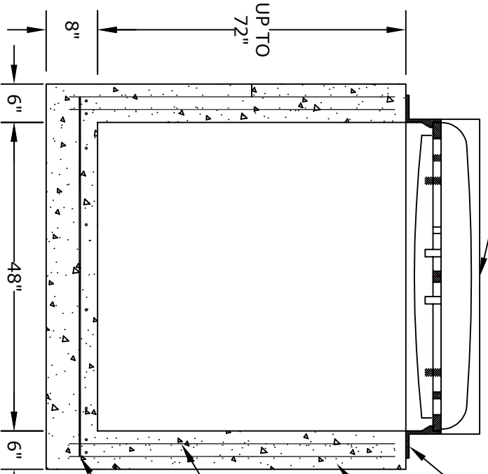
SECTION A
