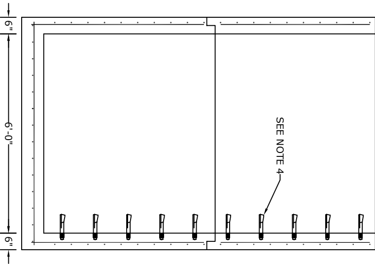
SECTION B
