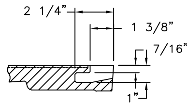
PICKHOLE DETAIL
