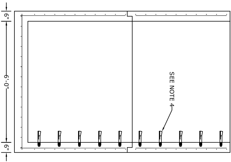
SECTION B
