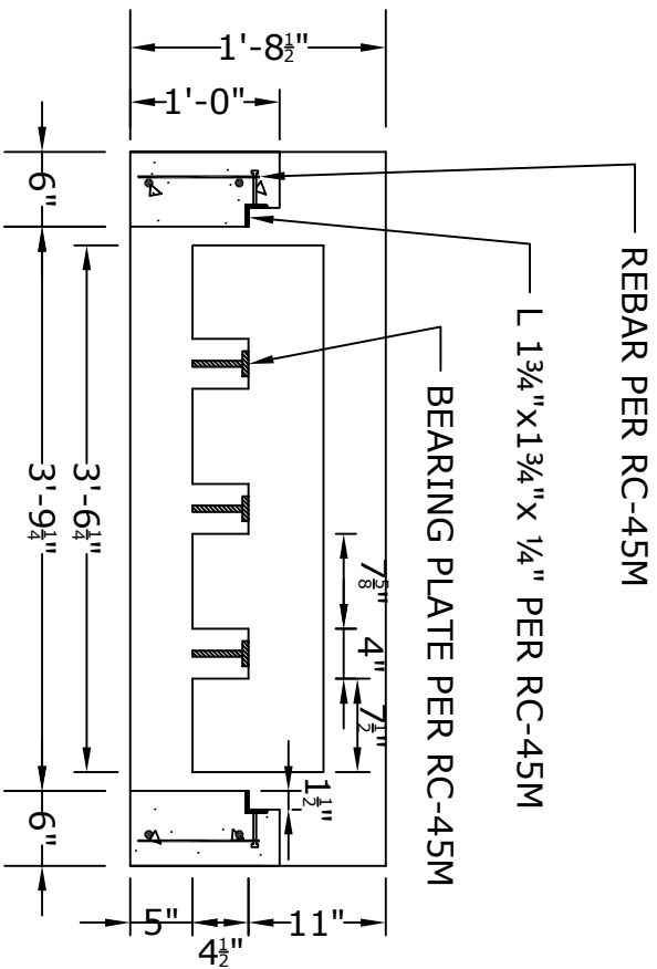
SECTION B
