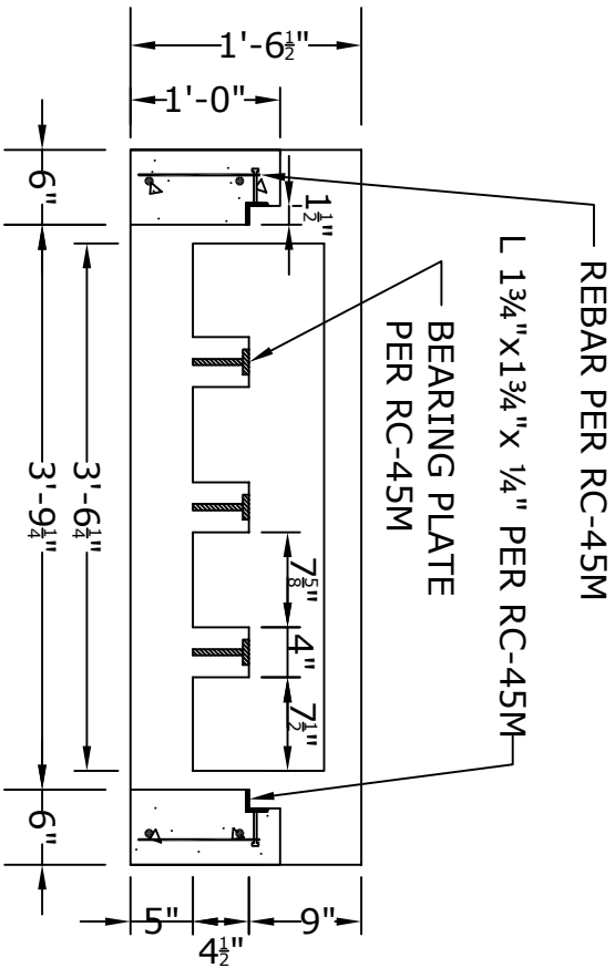
SECTION B
