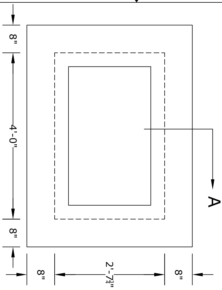
PLAN VIEW
