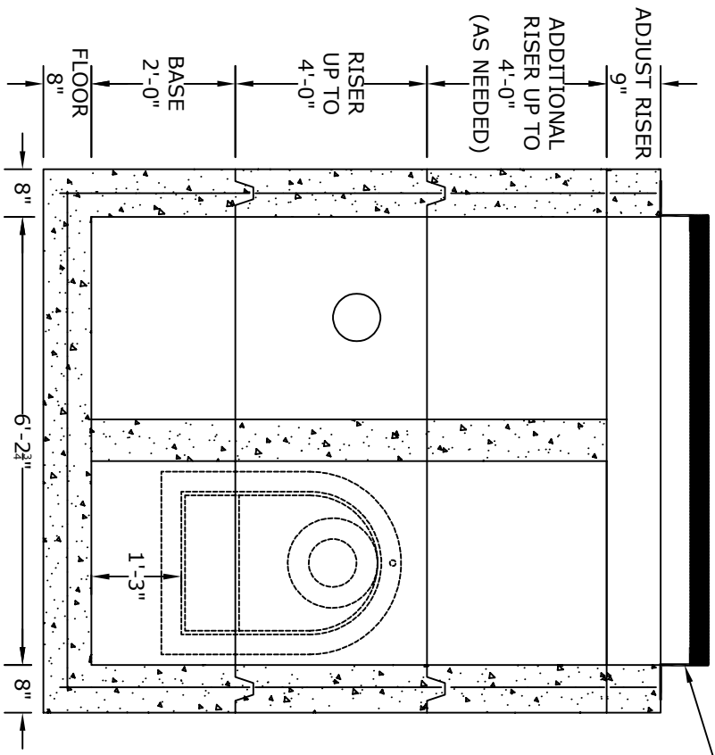
PLAN VIEW
