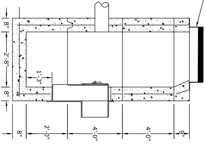
SECTION A
