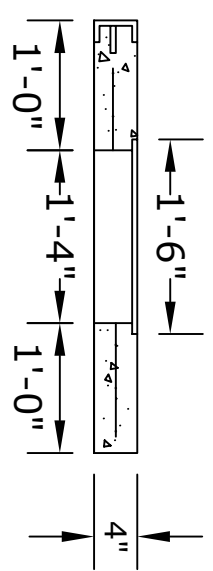
SECTION A
