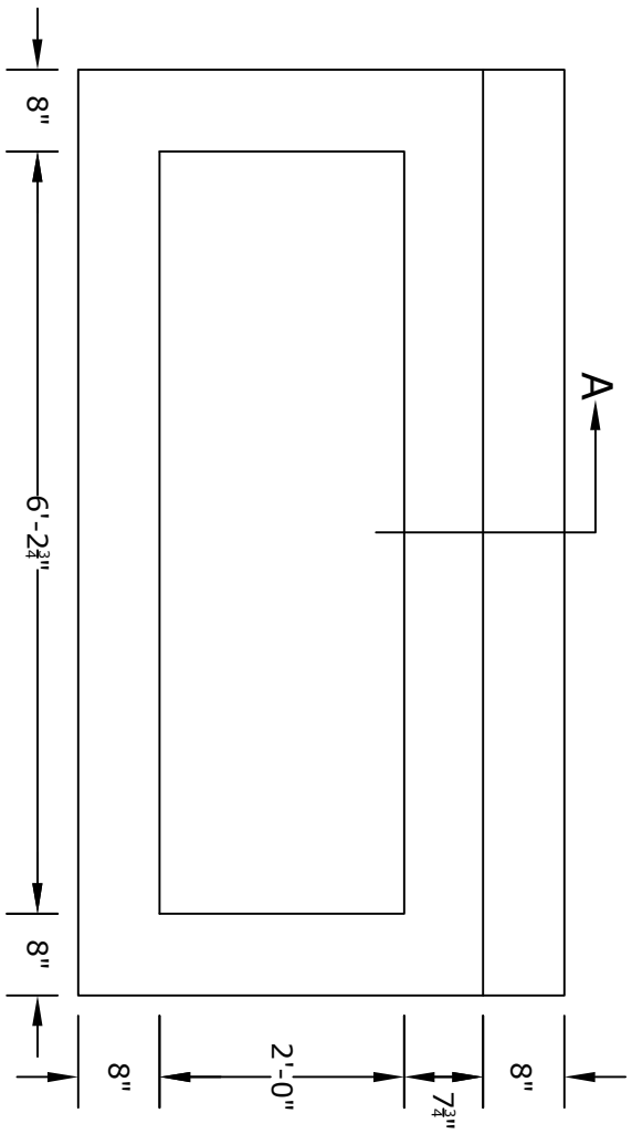
PLAN VIEW (SHOWN WITHOUT TOP SLAB)
