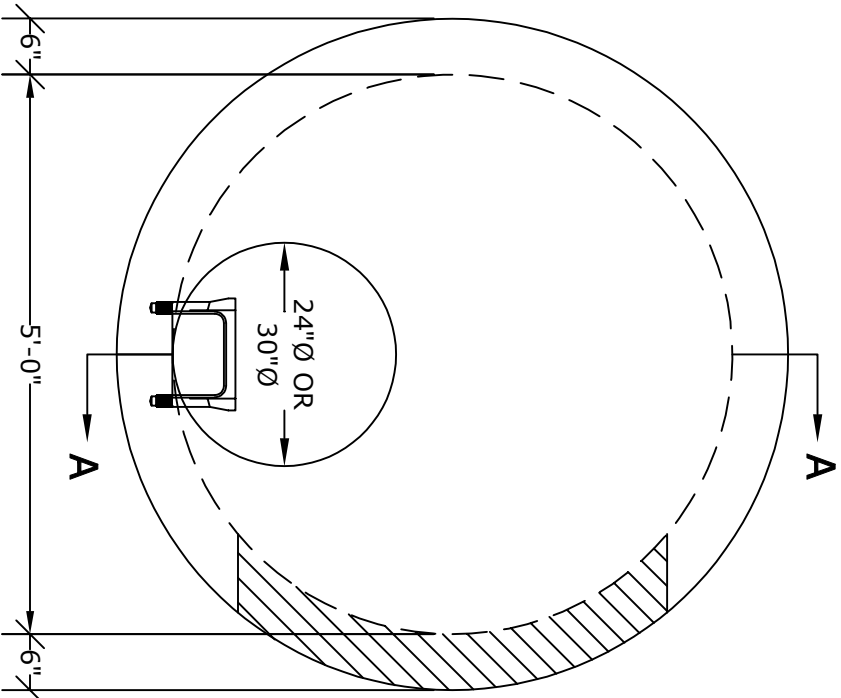
PLAN VIEW
