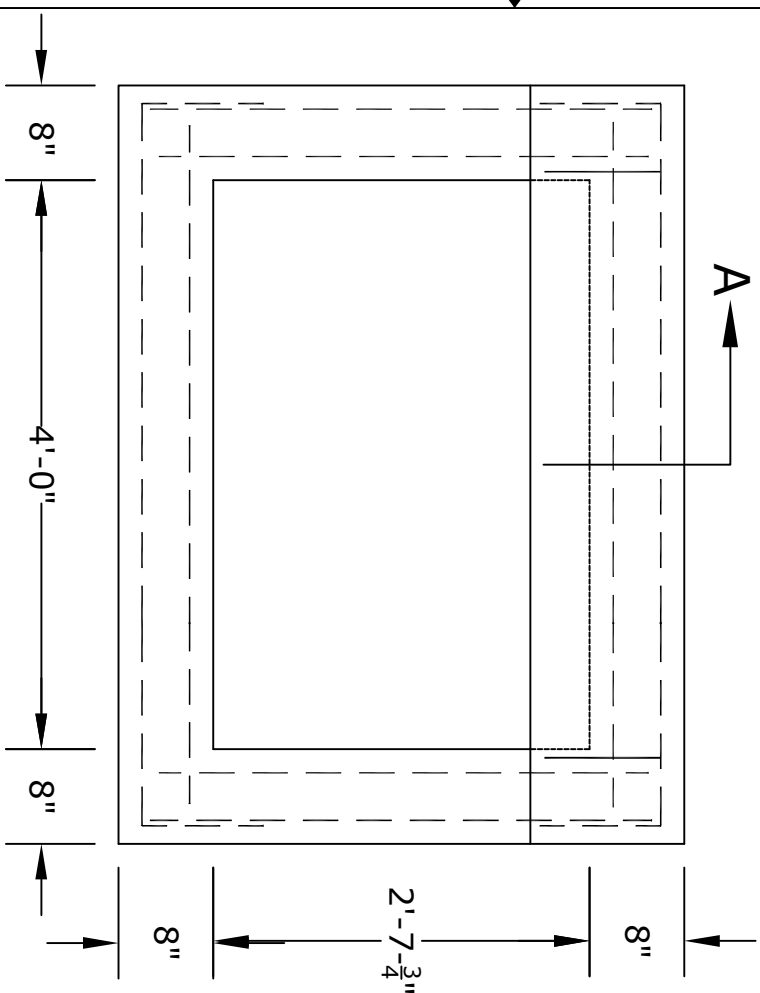
PLAN VIEW
