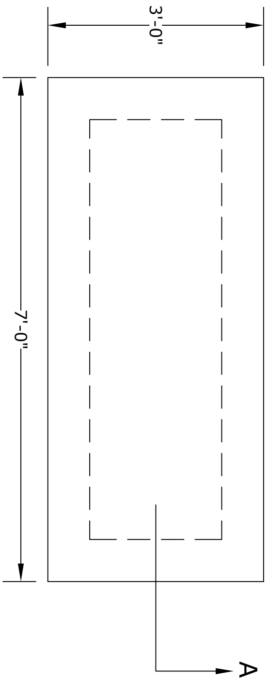
PLAN VIEW
