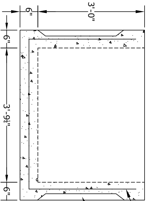
SECTION A
