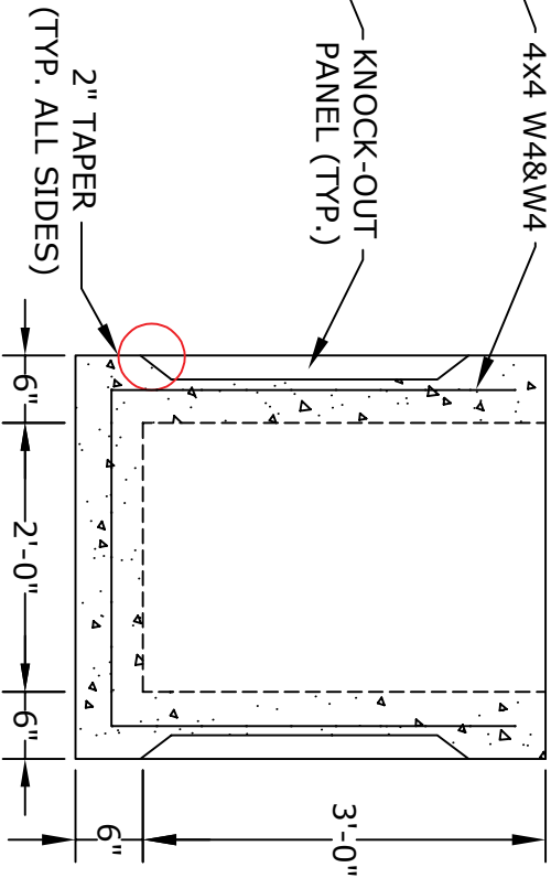
SECTION B
