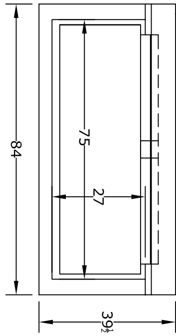
PLAN VIEW
