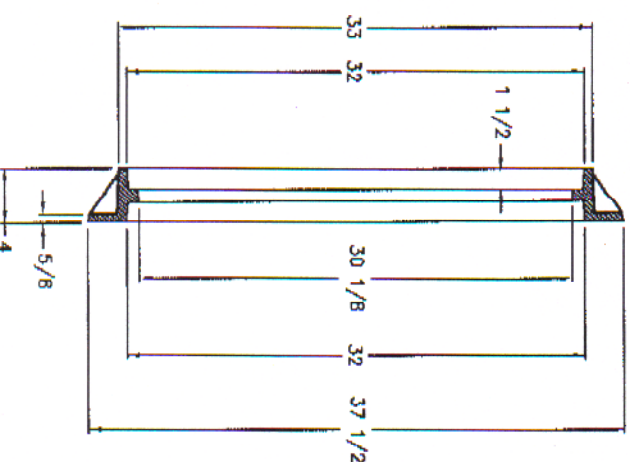
FRAME SECTION
