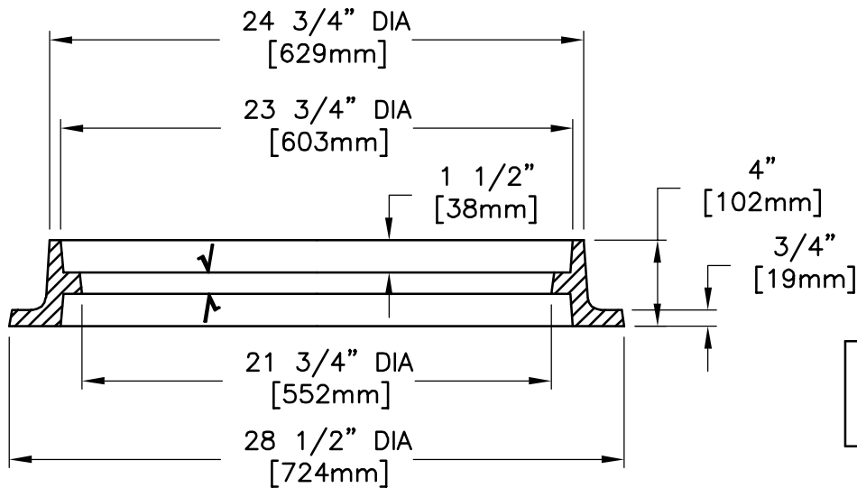
RING SECTION
