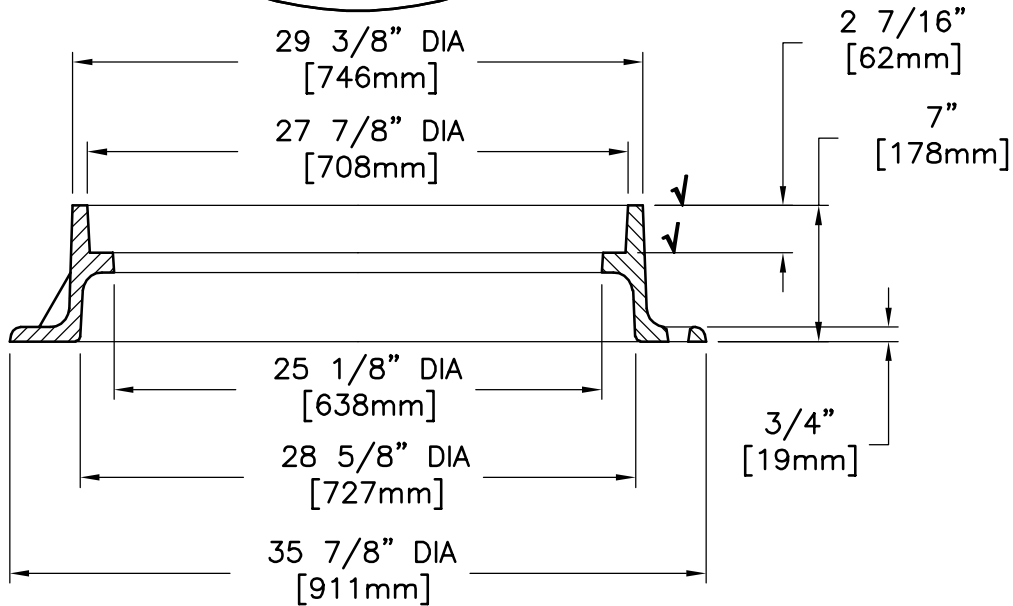
FRAME SECTION
