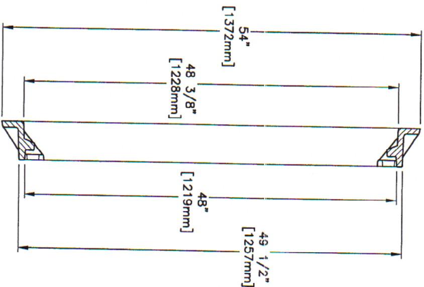
FRAME SECTION
