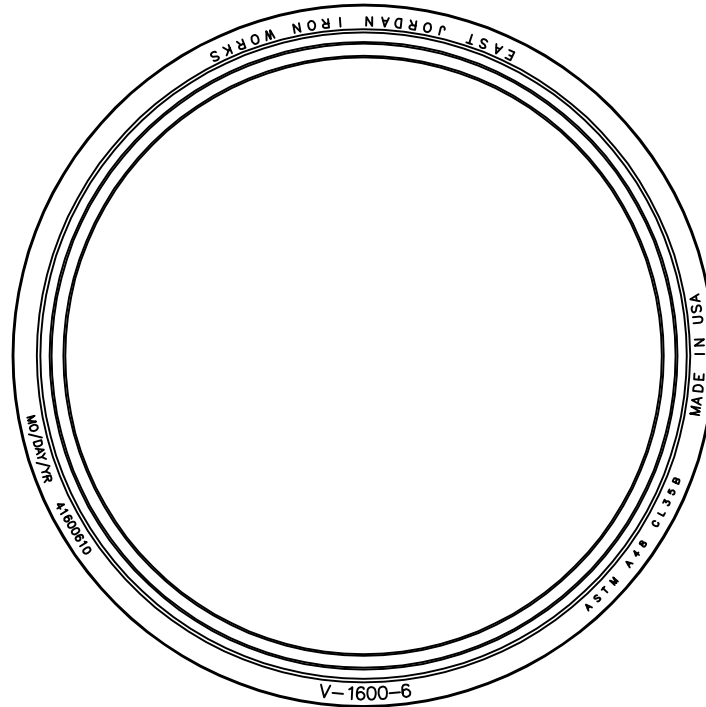
RING TOP VIEW
