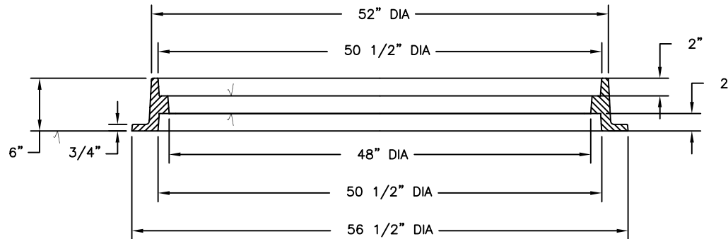
RING SECTION
