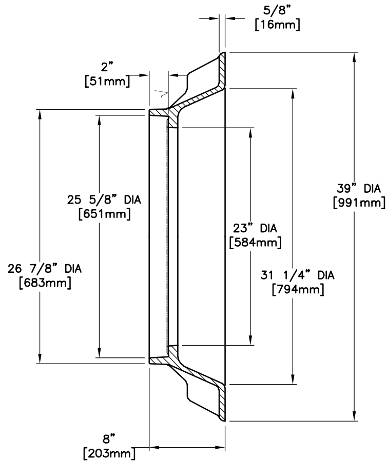
FRAME SECTION
