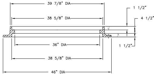
FRAME SECTION
