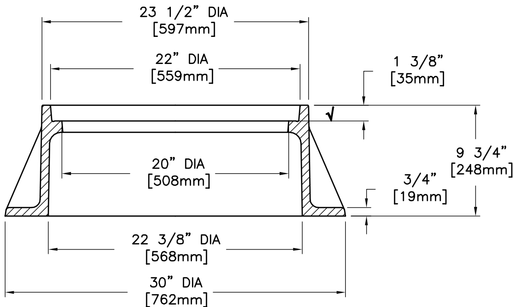
FRAME SECTION
