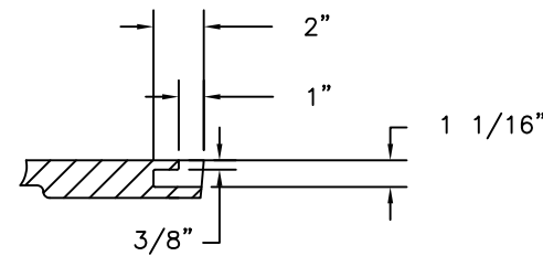
PICKHOLE DETAIL
