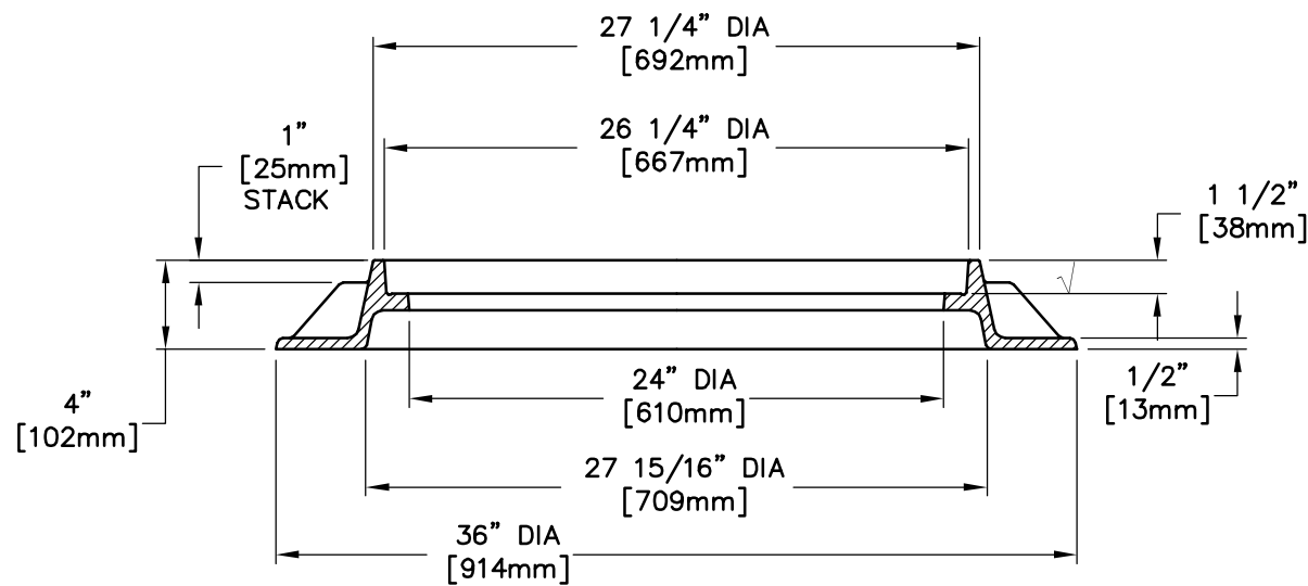
FRAME SECTION
