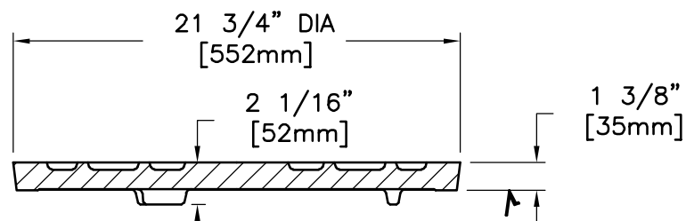
COVER SECTION
