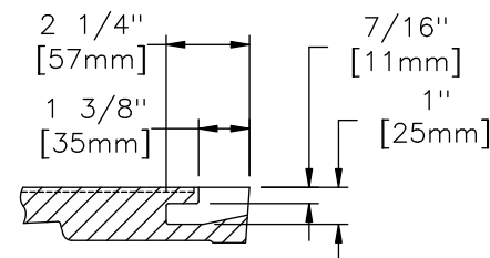
PICKHOLE & GROOVE DETAIL
