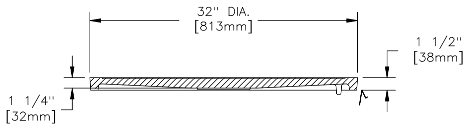
SECTION VIEW
