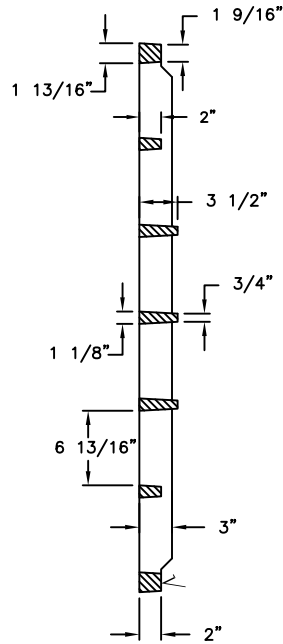
GRATE SECTION
