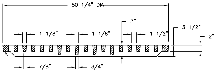
GRATE SECTION
