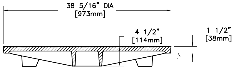
COVER SECTION
