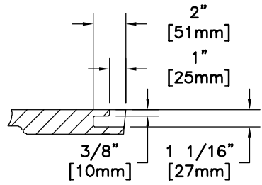
PICKHOLE DETAIL
