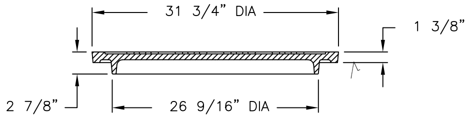
COVER SECTION
