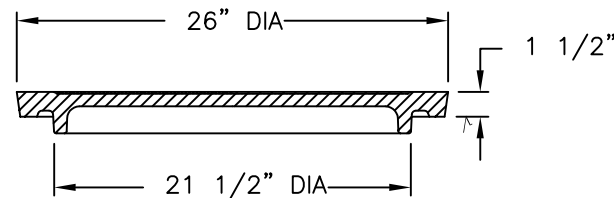
COVER SECTION
