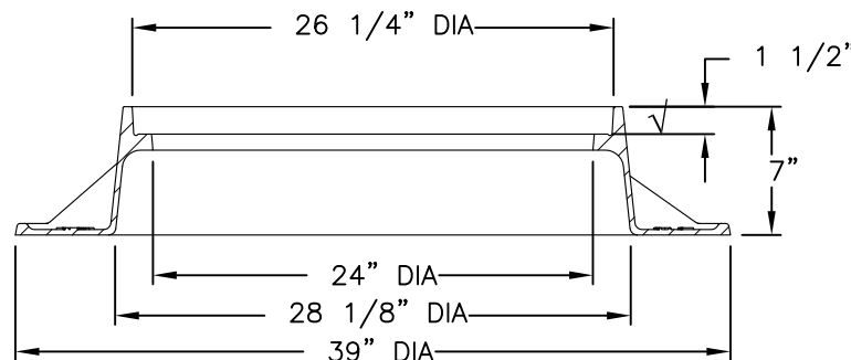
FRAME SECTION
