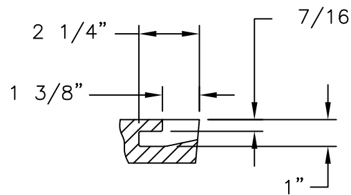
PICKHOLE DETAIL
