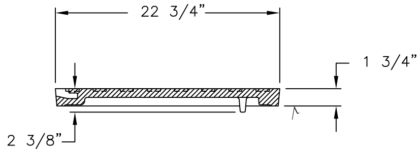
SECTION VIEW
