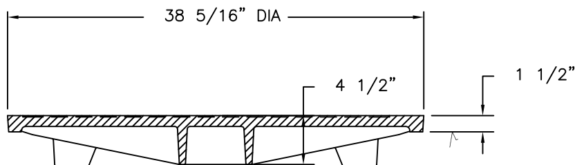
COVER SECTION
