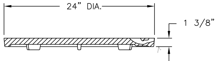
SECTION VIEW
