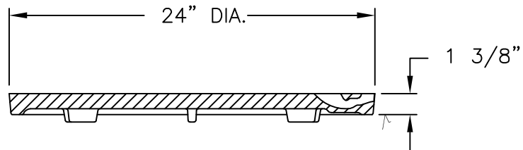
SECTION VIEW
