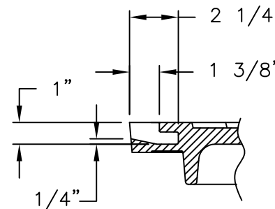
PICKHOLE DETAIL
