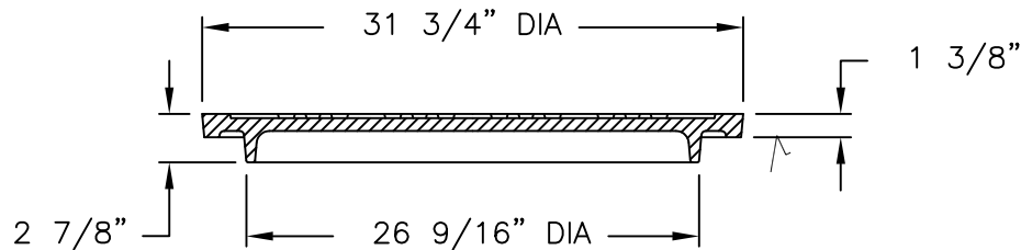
COVER SECTION
