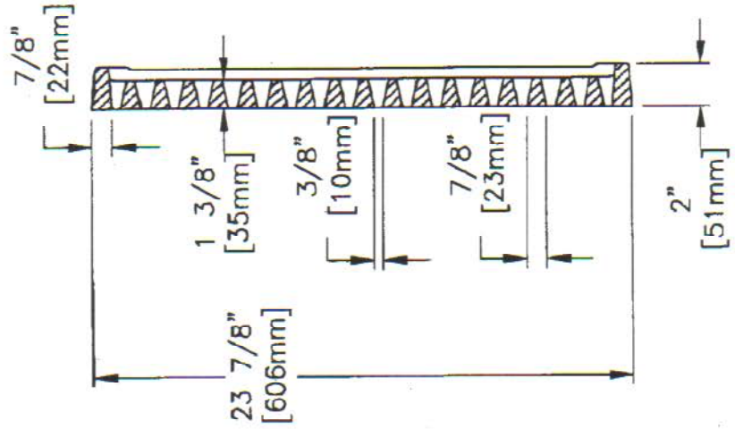
GRATE SECTION
