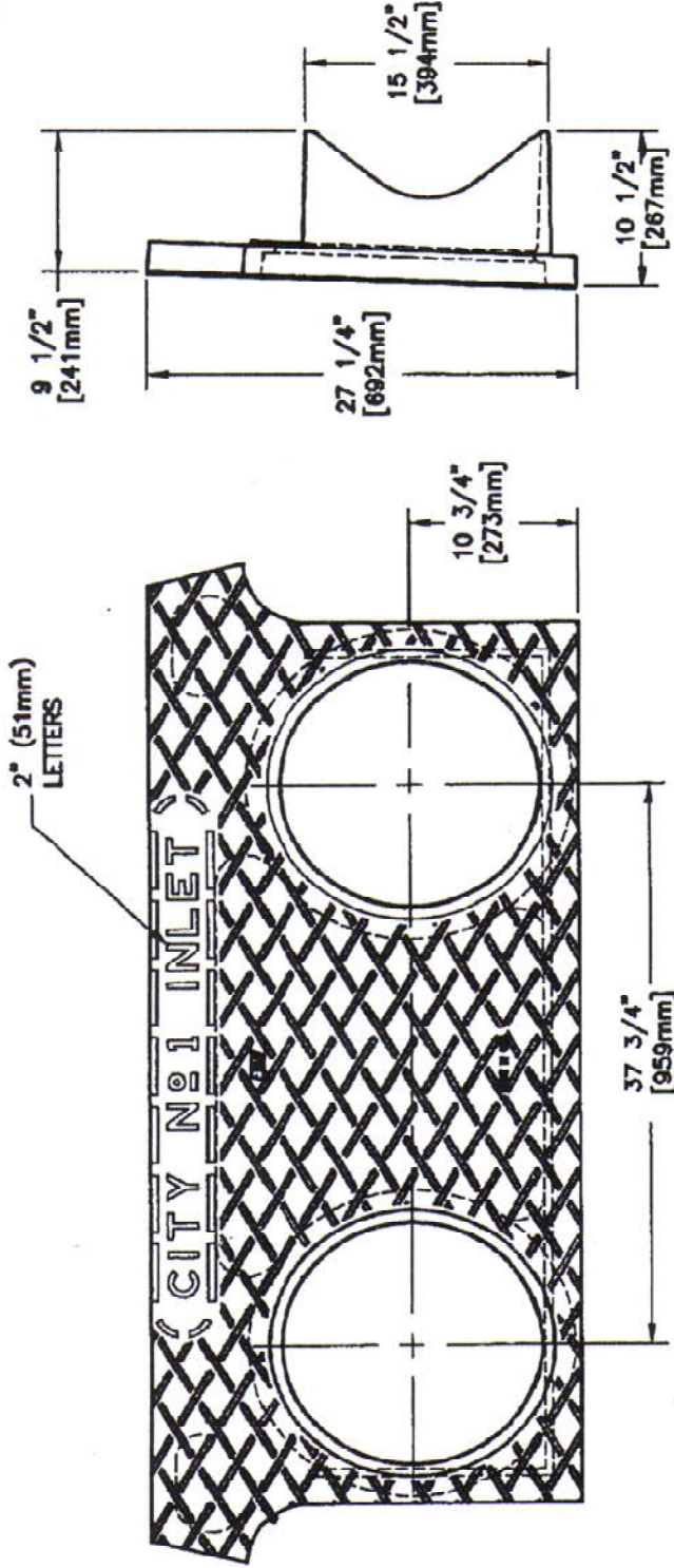
END VIEW
