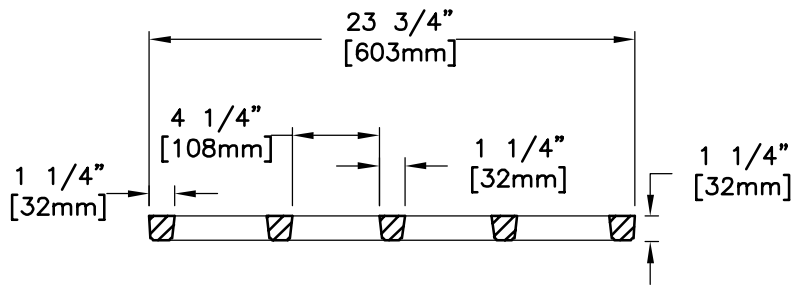
SECTION
