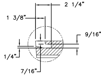
PICKHOLE DETAIL
