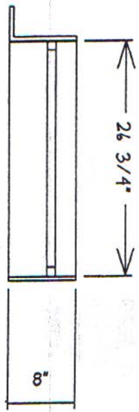
SECTION B-B
